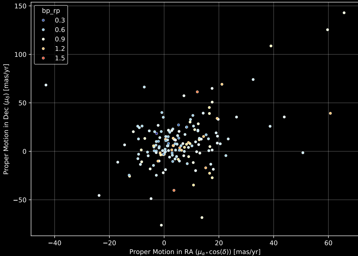
GALAH DR4 Field: [7215] Proper Motion Diagram (n= 167)
