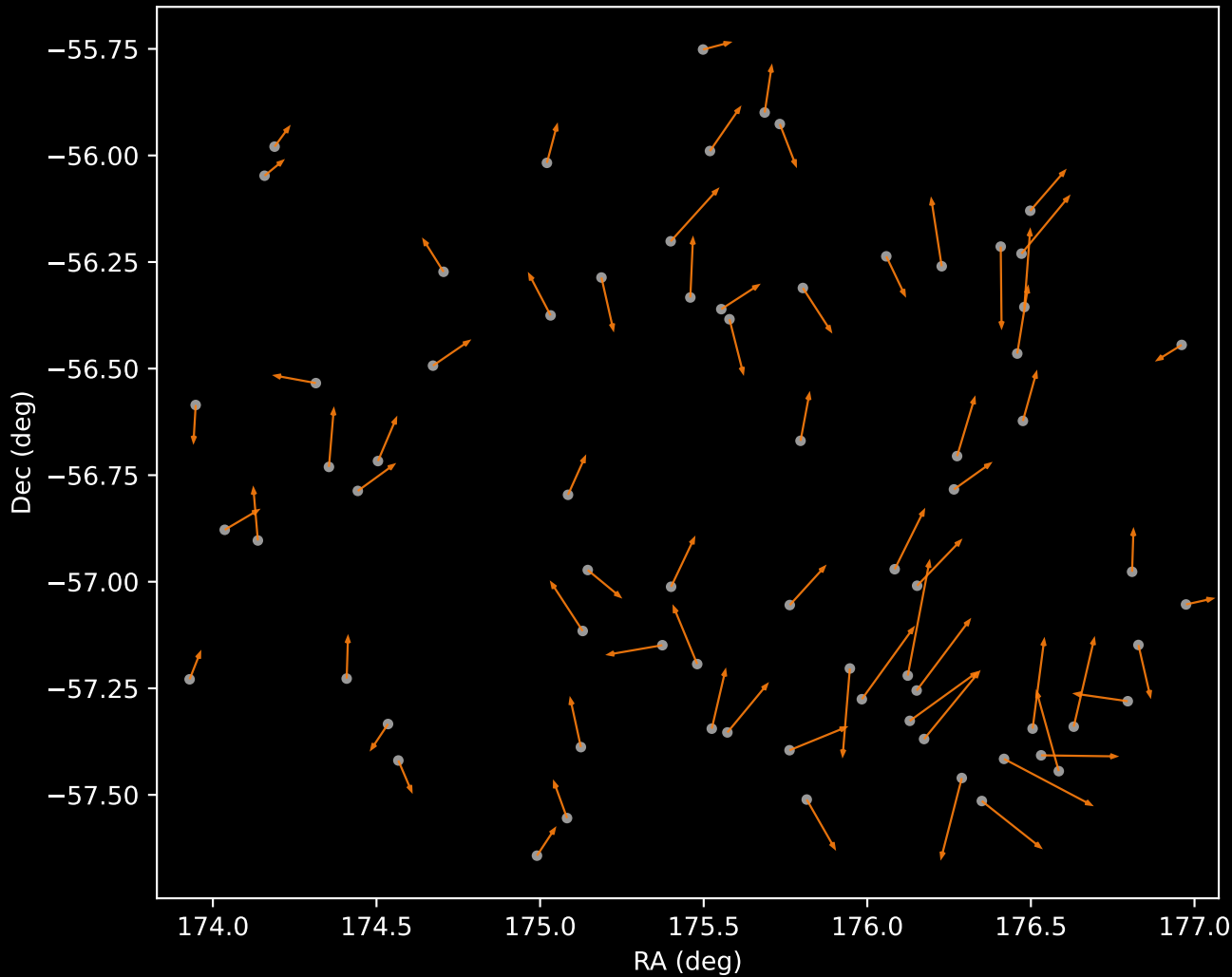
GALAH DR4 Cluster 2 Proper Motion Vectors (n=72)
