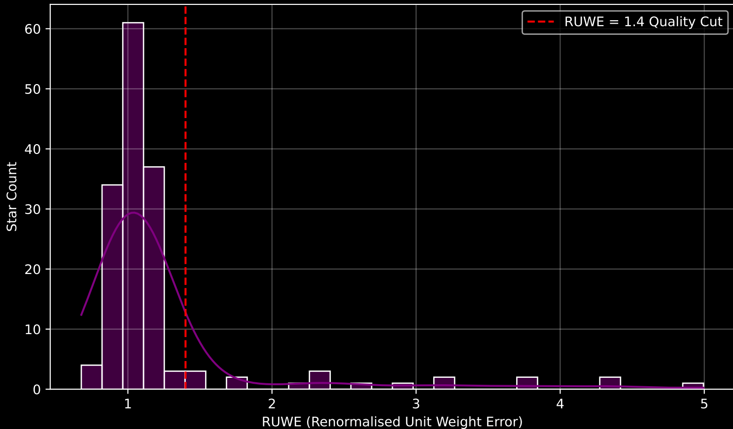
GALAH DR4 Field [7215] RUWE Distribution (n= 157)
