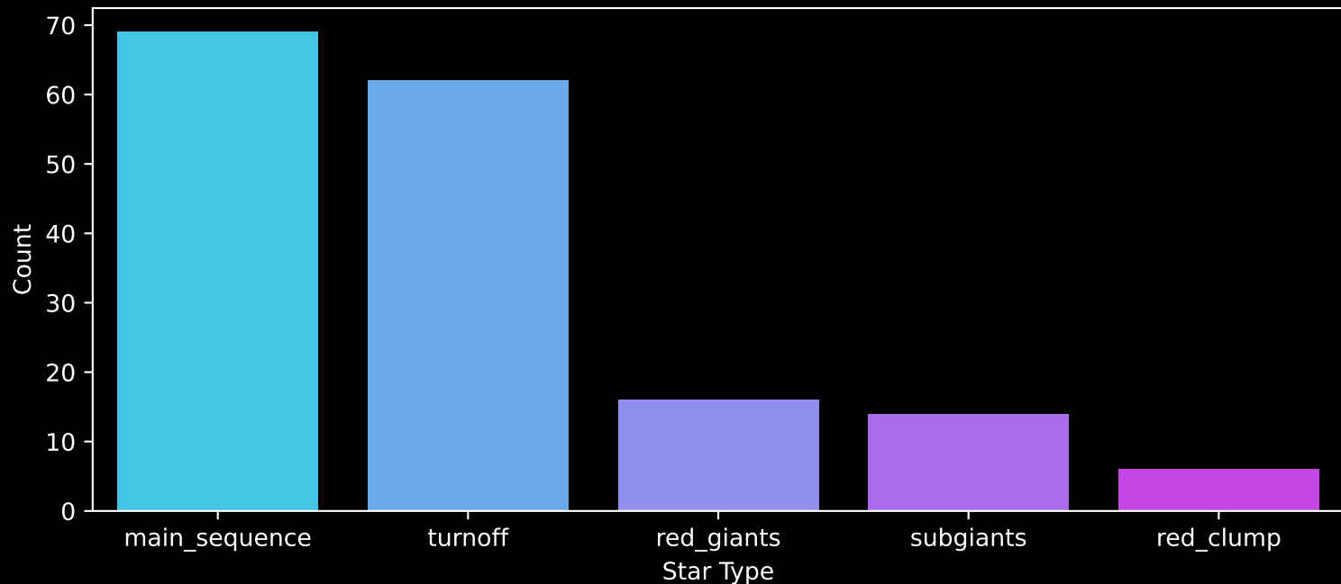
GALAH DR4 Field: [7215] Count plot of Star Type
