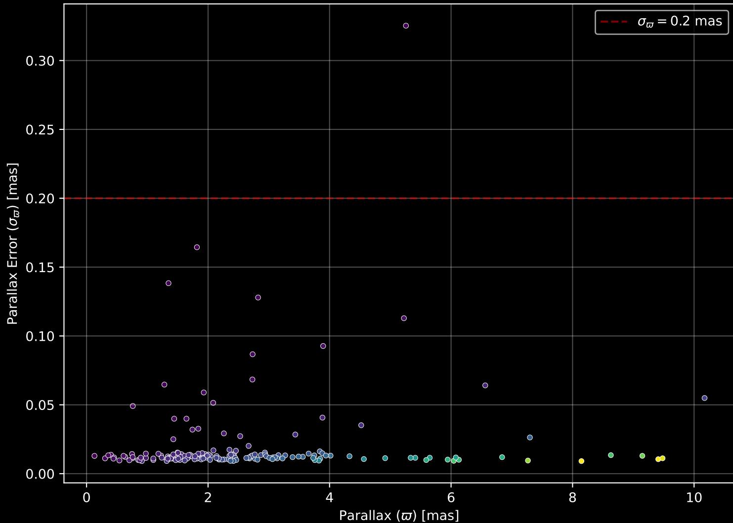
GALAH DR4 Field: [7215] Parallax Quality (n= 167)
