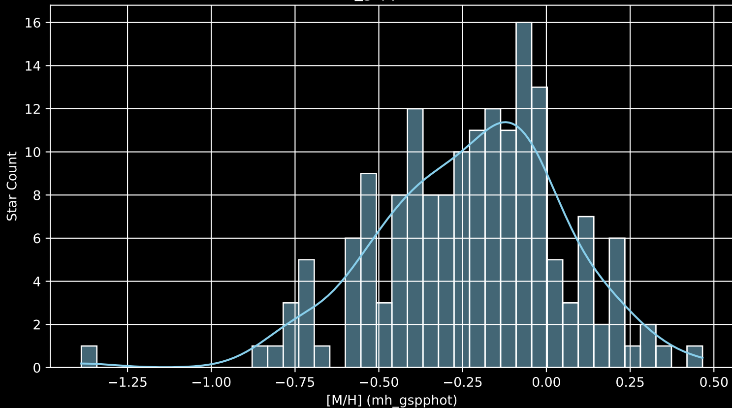
GALAH DR4 Field: [7215] [M/H] (mh_gspphot) (n= 167)
